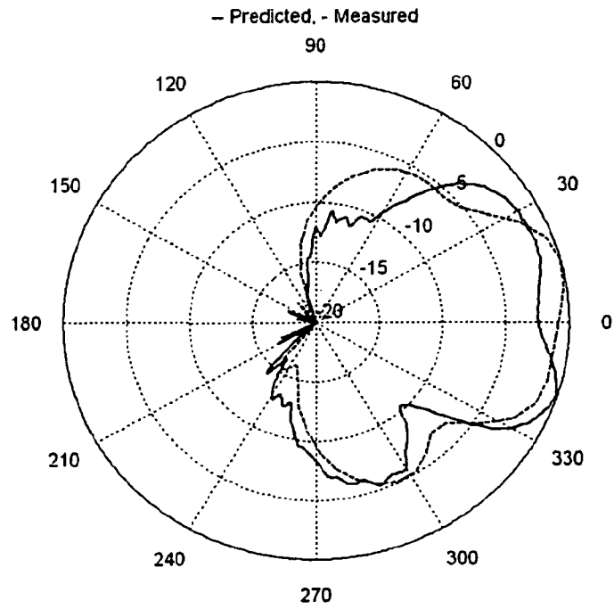
FIG. 3(a) E-Plane Radiation Pattern
