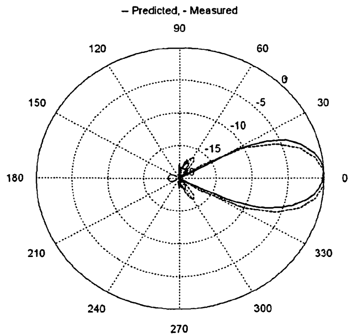
FIG. 3(b) H-Plane Radiation Pattern
